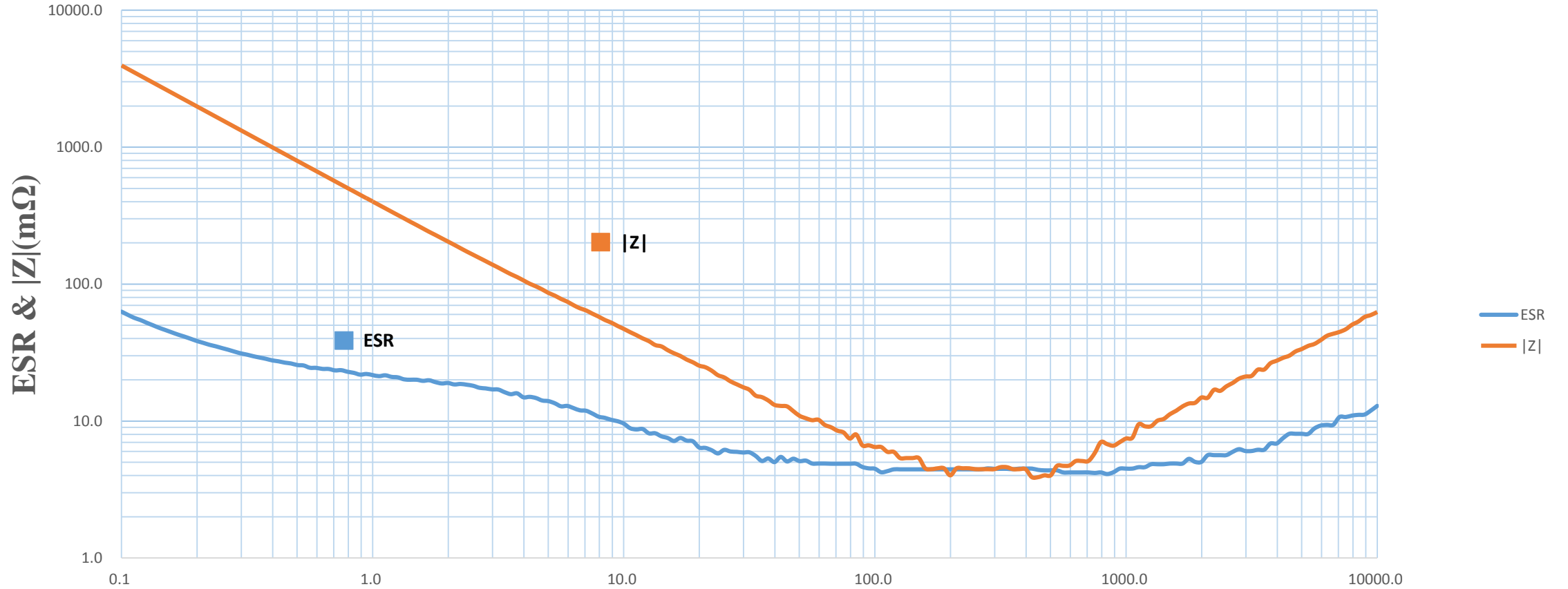
Frequency (KHz)
